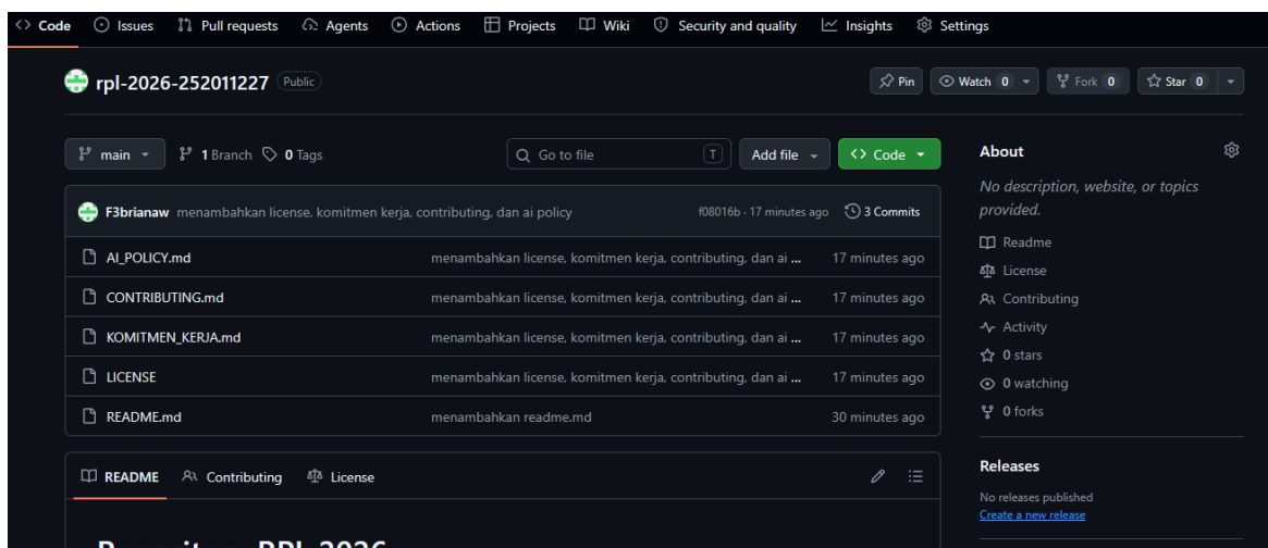
Gambar 7 repository rpl-2026-252011227
